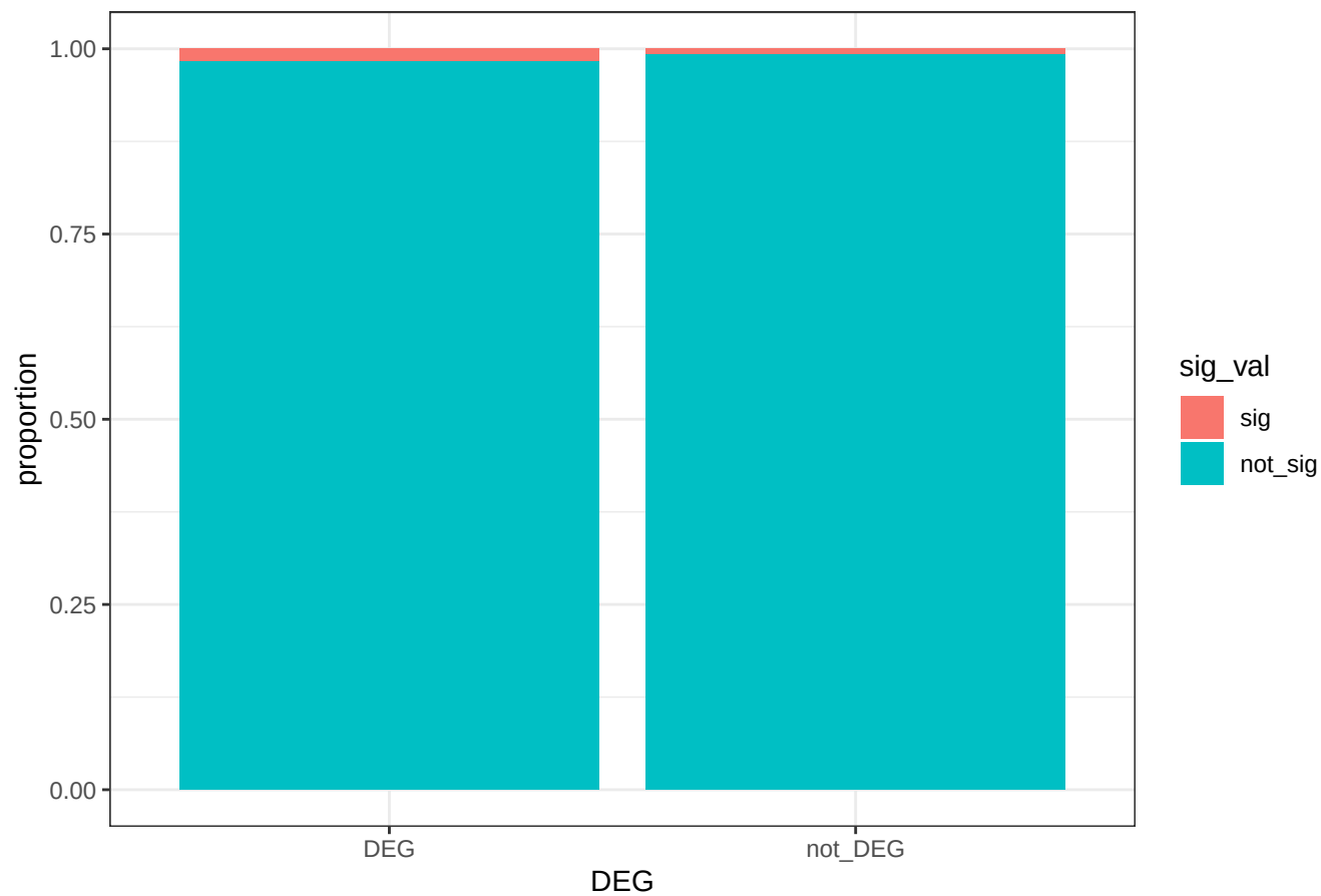
MTX DARs and not-DARs within 2kb of TSS of DEGs at 3 hours
